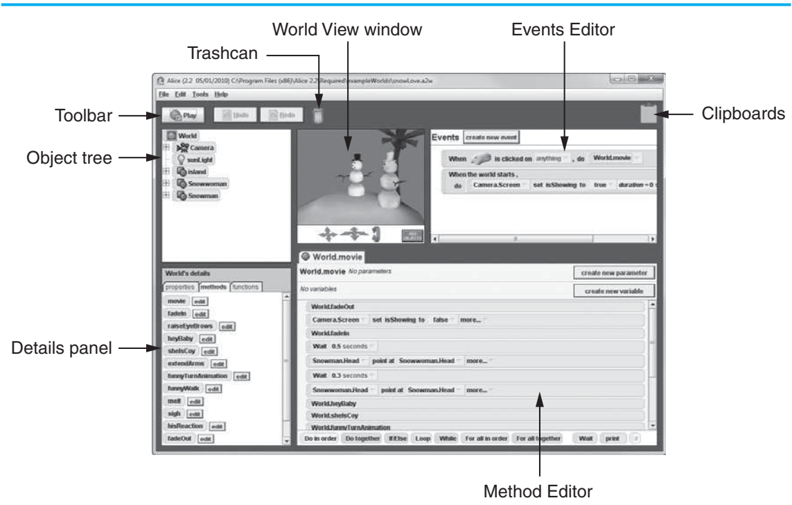
Figure A-3 Parts of the Alice environment
